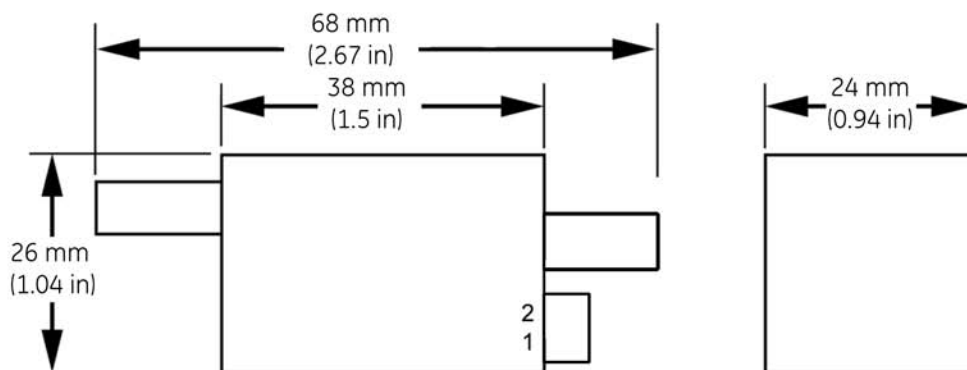
FIGURE 2: MODULE DIMENSIONS
