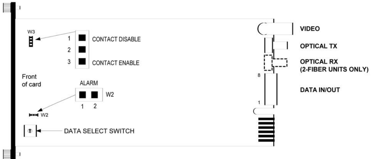
FIGURE 4: RACK-MOUNT TRANSMITTER
